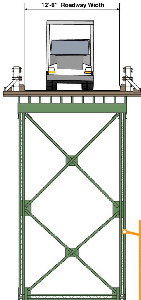
Existing Bridge
