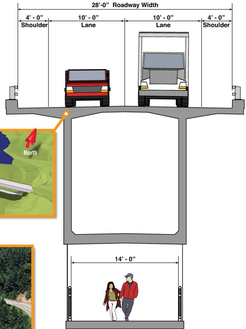
Proposed Bridge
